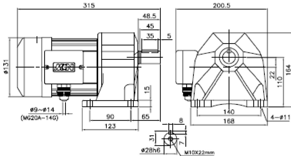
3 Phase Gear Motor Horizontal Type
