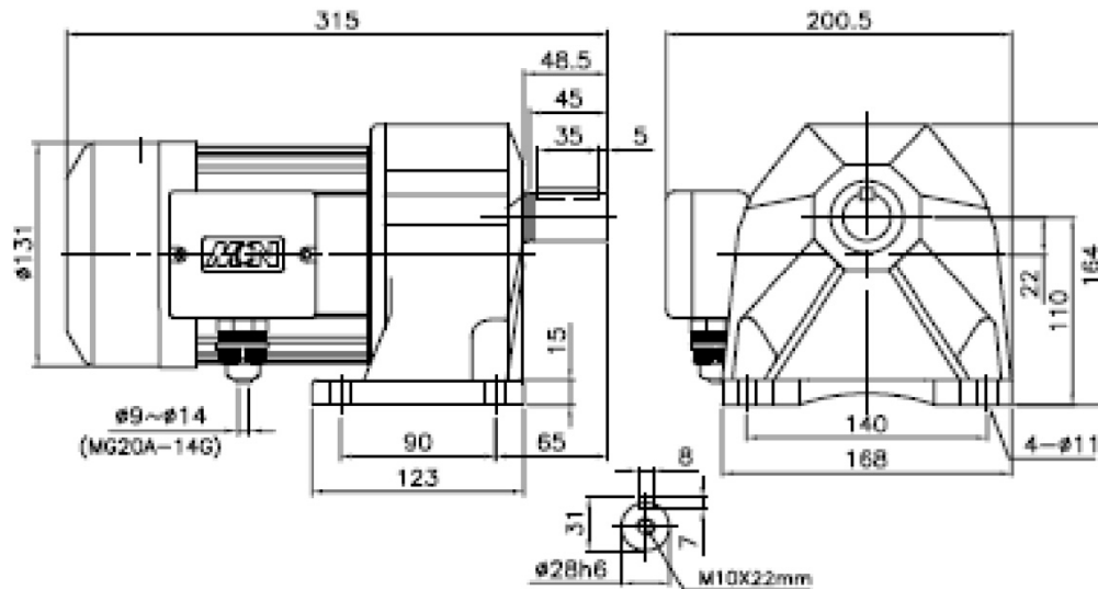
3 Phase Gear Motor Horizontal Type
